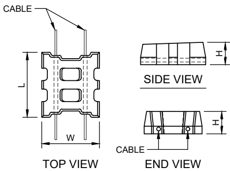
TAPERED OPEN CELL BLOCK
