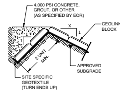
TOP OF SLOPE TERMINATION DETAIL
