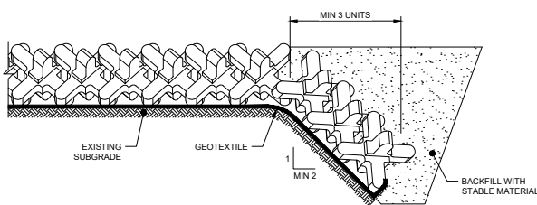
FLANK TERMINATION
