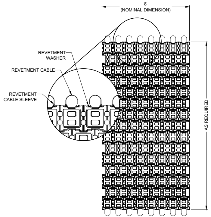
TYPICAL MAT PLAN
