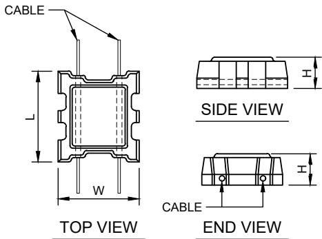
CLOSED CELL BLOCK
