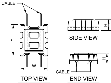
OPEN CELL BLOCK
