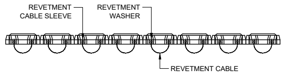
TYPICAL MAT END VIEW
