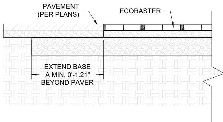
ECORASTER ASPHALT EDGE RESTRAINT DETAIL
