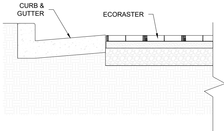
ECORASTER GUTTER EDGE RESTRAINT DETAIL
