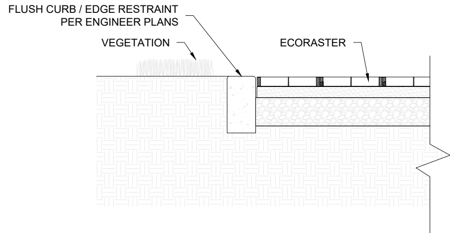
ECORASTER W/ EDGE RESTRAINT & GRASS DETAIL
