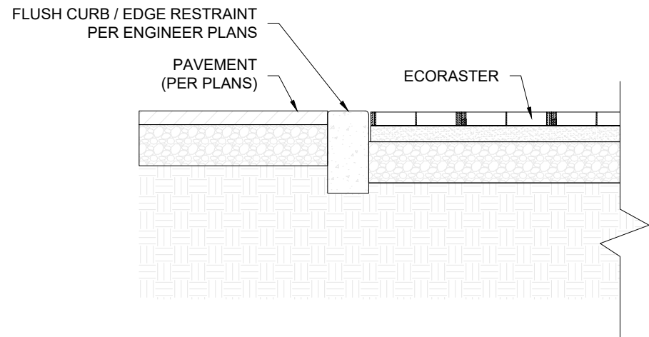
ECORASTER W/ EDGE RESTRAINT & PAVEMENT DETAIL
