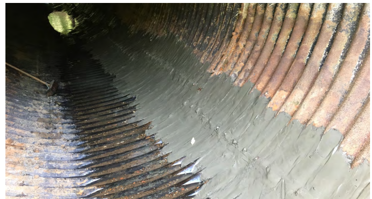
Smoothing over protrusions using grout
